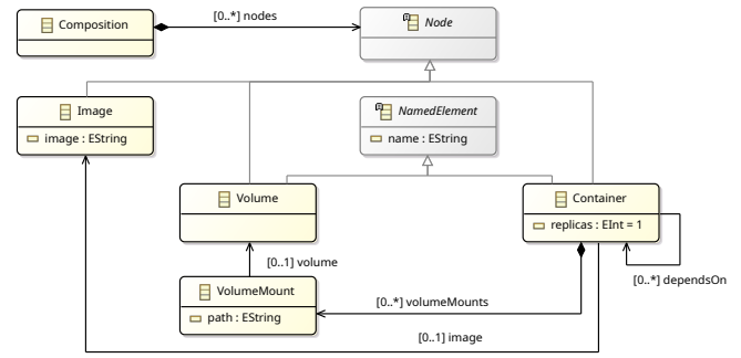
Figure 1: Class diagram for the Containers metamodel
