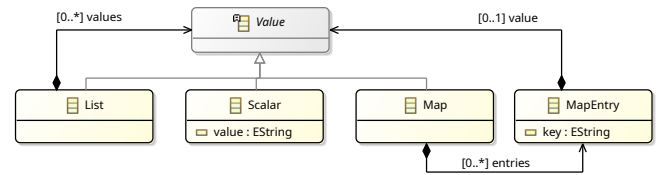
Figure 2: Class diagram for the MiniYAML metamodel
